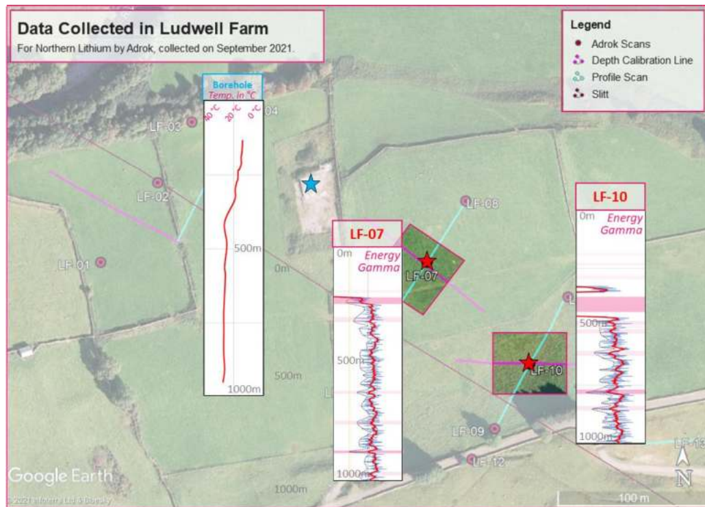
Figure 6 Eastgate (Ludwell Farm) results show LF-10 has highest energy reflection readings with greatest thermal impact responses and higher confidence, at 380-440m. By studying the rest of the sites and processing the profile scans, Adrok would be able to provide a more in-depth explanation of the thermal dynamics in the subsurface of Ludwell Farm, as well as tying it together with our flow readings. This would allow for a robust interpretation of the hot lithium brines.
