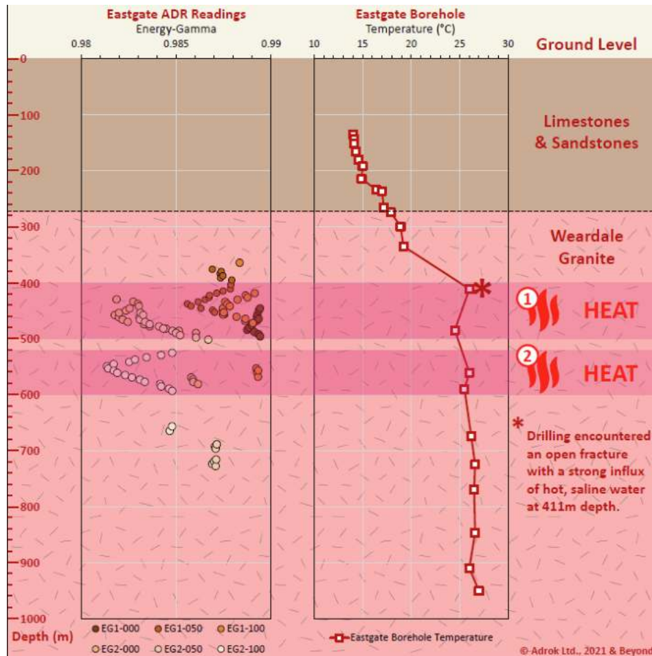
Figure 5 Eastgate 2 site E-gamma readings in NE England shown on left-hand graph versus observed temperature at Eastgate 2 site physical drillhole in NE England right-graph alongside lithology log on right-hand-side (observed temperature data from PB Power et al 2005). EG1-000 to EG2-100 signify the site names where ADR readings were collected.
